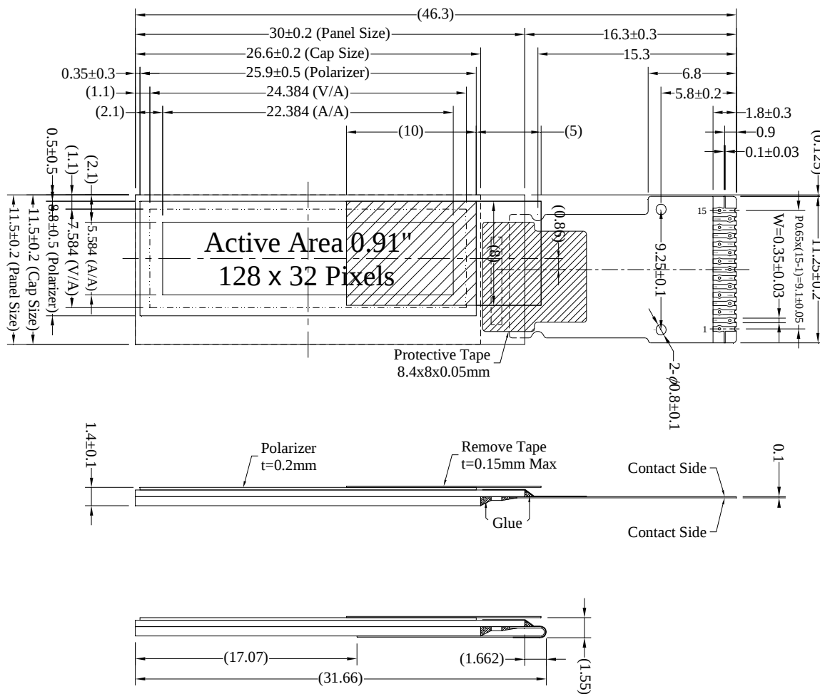
(Reference Mechanical Design)
